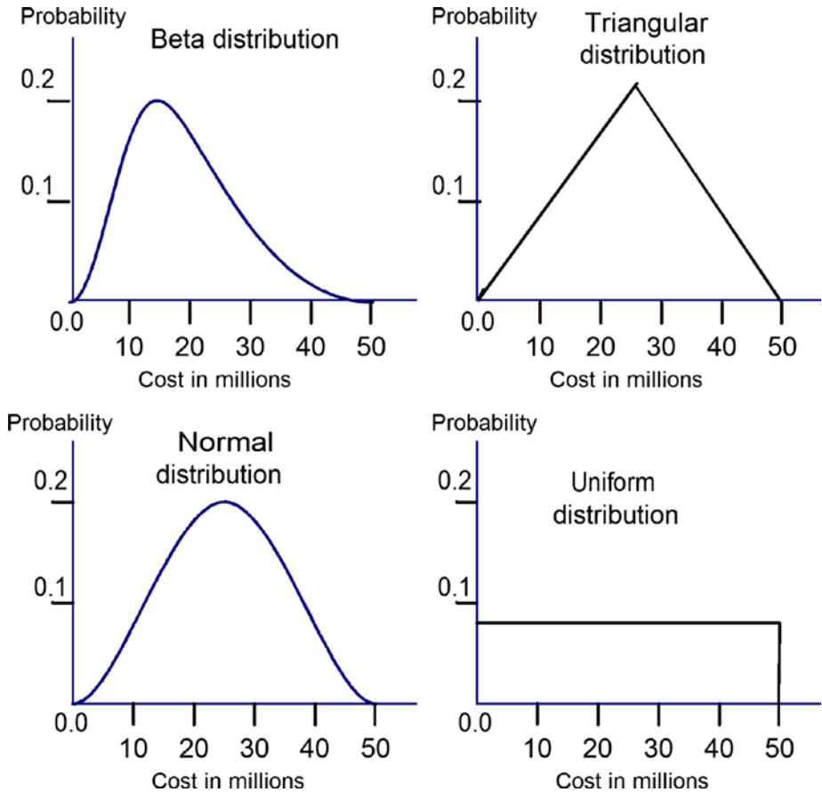
Figure 11-2. Examples of probability distributions commonly used in quantitative risk analysis
