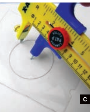
Fig. A: Calipers give an accurate inner diameter of your yo-yo. Fig. B: Set the compass cutter to match the inner radius. Fig. C: Cut the side cap out of sheet plastic. Fig. D: Measure your coin cell battery, then lightly scribe
