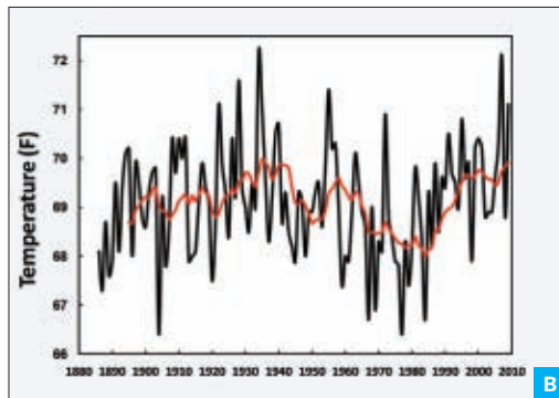
Fig. A: Preliminary annual temperature measured by the National Weather Service at San Antonio, Texas, from 1885 to 2009. Fig. B: Figure A with a superimposed 10-year running average that more clearly reveals patterns and trends in the data. Fig. C: Figure A with a superimposed mean and linear trend (given by the equation at top) and a color-coded background.
