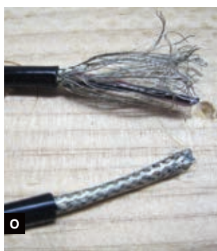
Fig. N: Solder bobbin wires to pins. Fig. O: Prepare a short length of shielded cable by removing a bit of insulation from each end. Fig. P: One end of the cable was soldered to the pins and the other to the lugs of the phono jack.
