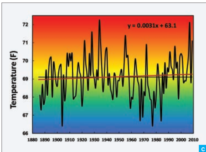
Fig. A: Preliminary annual temperature measured by the National Weather Service at San Antonio, Texas, from 1885 to 2009. Fig. B: Figure A with a superimposed 10-year running average that more clearly reveals patterns and trends in the data. Fig. C: Figure A with a superimposed mean and linear trend (given by the equation at top) and a color-coded background.
