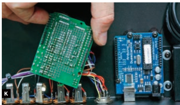
ProtoShield (2), mic connector from Headgear unit (3), mono mic jacks out to PreSonus FireStudio preamp (4). Fig. K: Electronics layout, with ProtoShield lifted to reveal Arduino Duemilanove.
