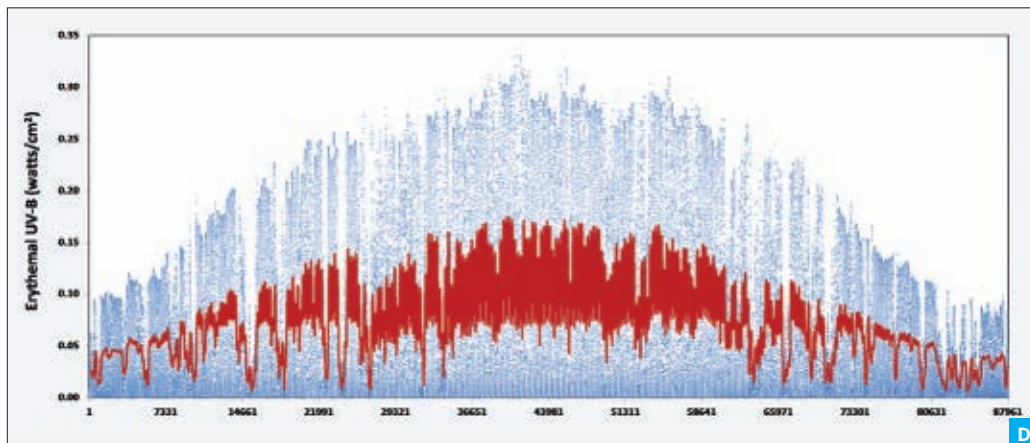
Fig. D: The 87,977 readings (blue) every three minutes and the seven-day running average (red) of solar ultraviolet radiation during 2009 measured by the USDA instrument in Figure E. Because of a few days of data outages, it wasn't possible to label the y-axis with dates. That's why I call this chart a "work in progress." Fig. E: UV-B data from this U.S. Department of Agriculture radiometer at Texas Lutheran University at Seguin, Texas, are online (see text).
