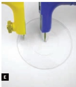
a matching circle in the center of the cap. Fig. E: To mark the LED positions, scribe 2 opposite arcs in between the battery circle and the cap's edge. Then lay a straightedge across the center. Fig. F: The cap with LED holes drilled.
