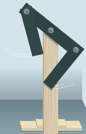
Simple or Chaotic: Rott's Pendulum
