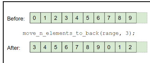
Moving the first three elements to back of a range
