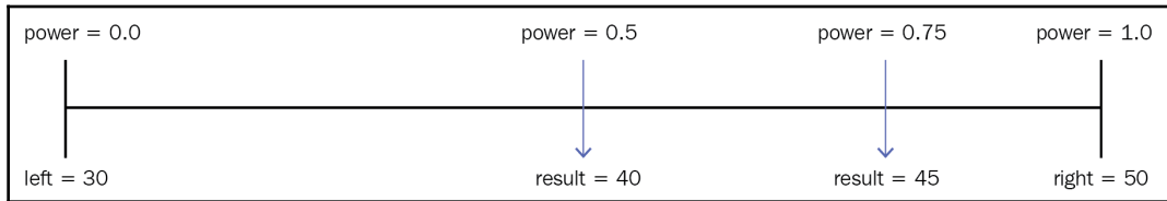
Illustration of interpolation function
