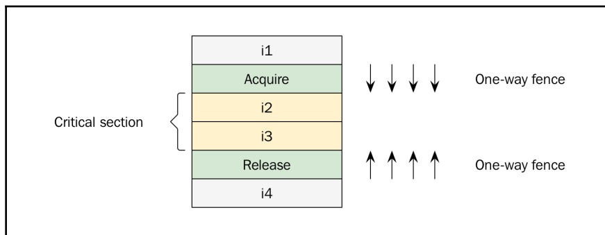
The one-way fences limit the reordering of the instructions
