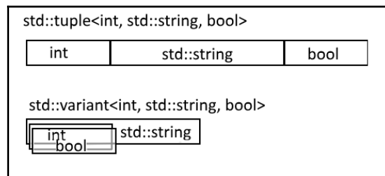
Tuple of types versus variant of types
