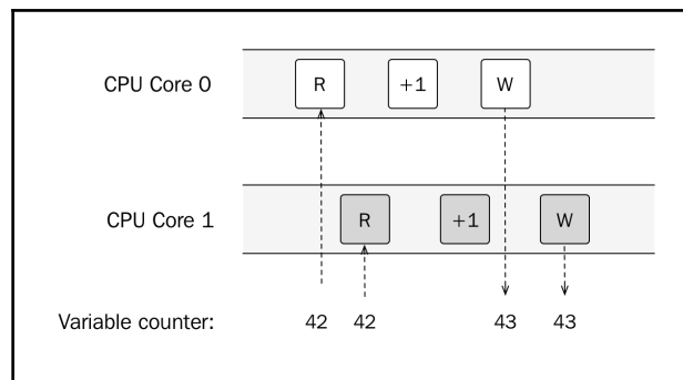
The two threads are both incrementing the same shared variable
