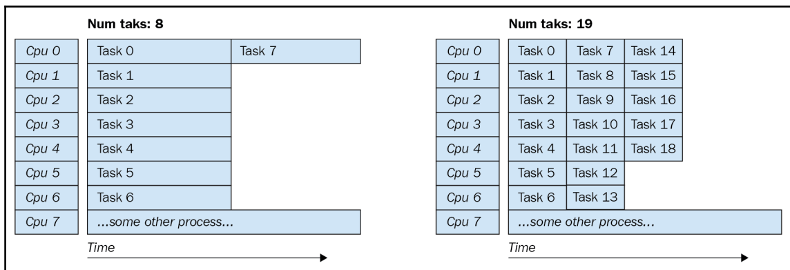
Possible scenarios where computation time is proportional to chunk size
