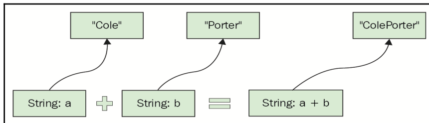
Accumulating two strings into a new string
