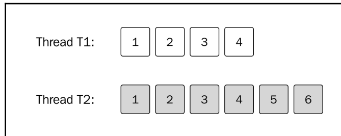
Two separate sequences of instructions executed in two threads labeled T1 and T2
