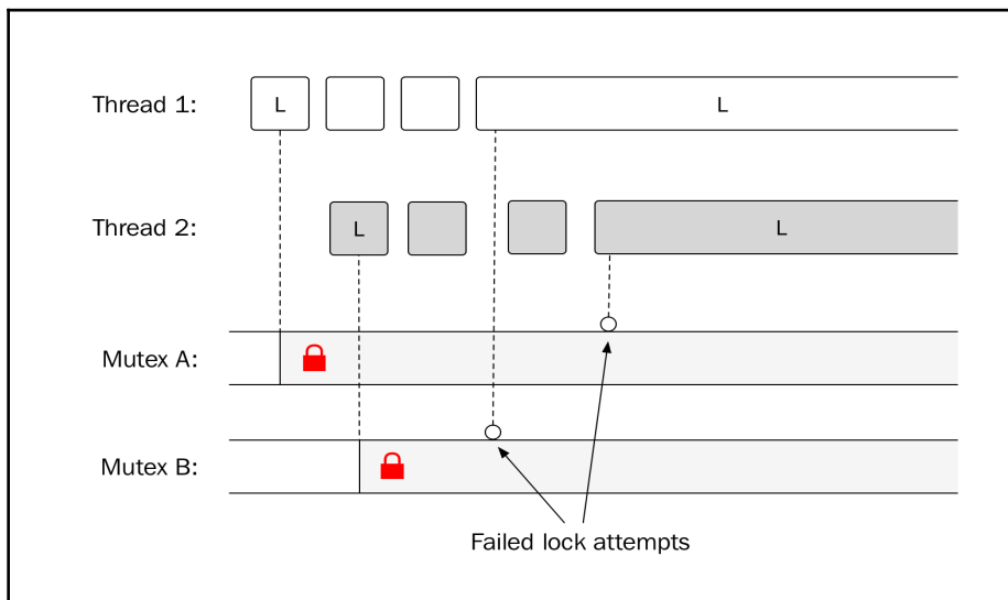
Example of a deadlock state. Thread 1 and Thread 2 are waiting for each other to release their locks, respectively
