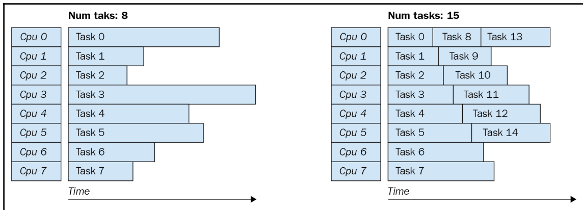
Possible scenarios where computation time is not proportional to chunk size
