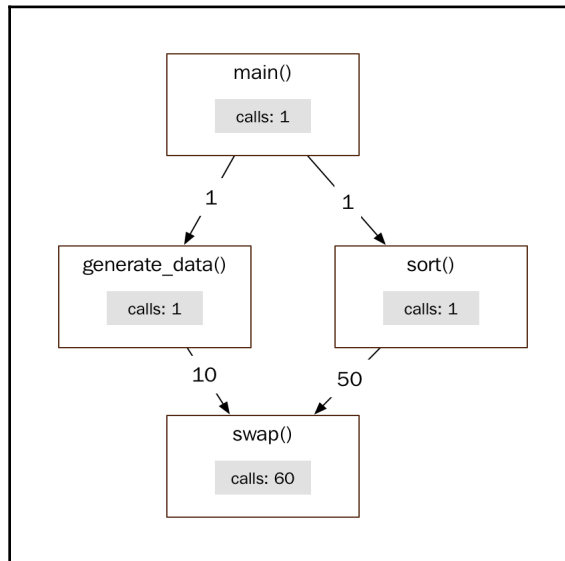
Example of a call graph
