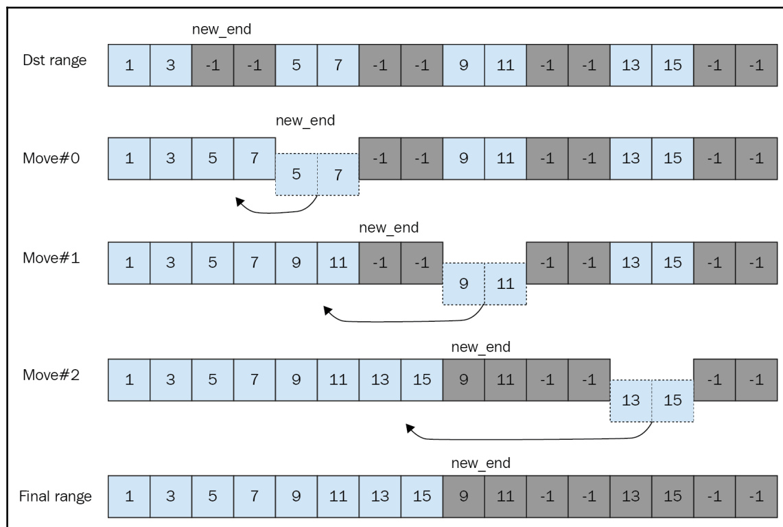
Merge sparse range into a continuous range
