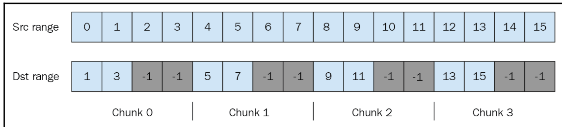
Sparse destination range after first step of conditional copy
