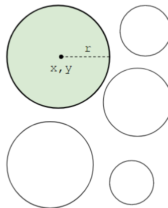
Circles of different size and position
