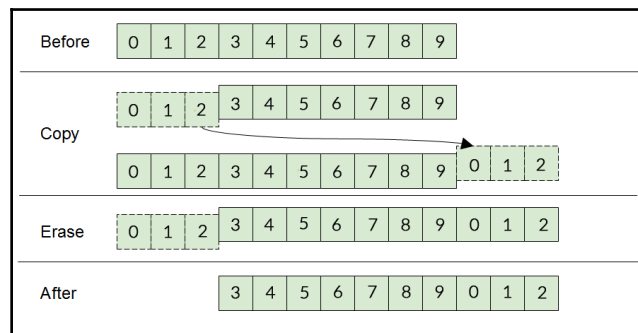
Allocating and deallocating in order to move elements to back of range
