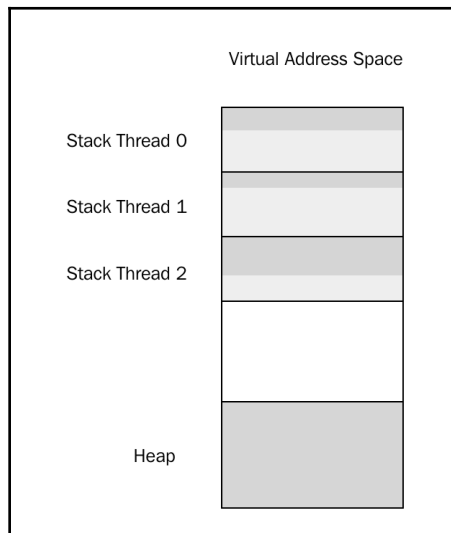
A possible layout of the virtual address space for a process
