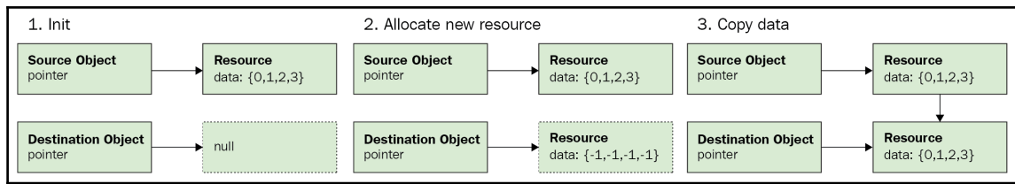
Copying an object with resources
