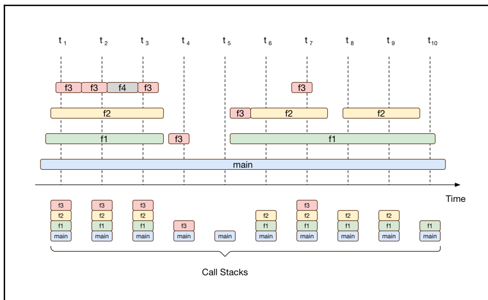
Example of a sampling profiler session
