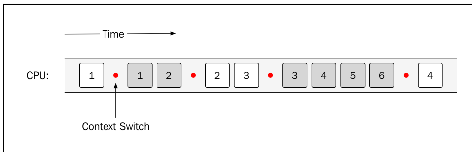
A possible execution of two threads which are being scheduled on a single core. The red dots indicate context switches
