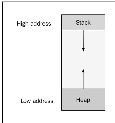
An address space of a process. The stack and the heap grows in opposite directions.
