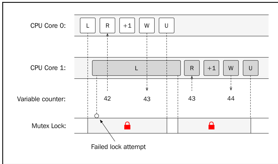
The mutex lock is protecting the critical section and avoids the data races on the counter variable
