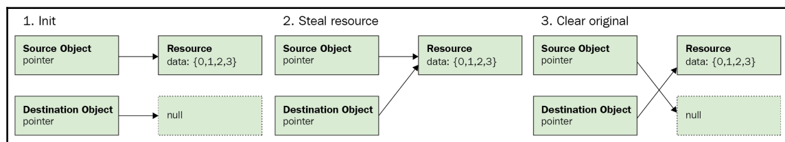
Moving resources from one object to another
