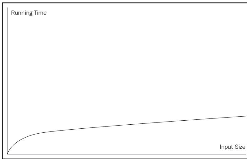
Logarithmic growth rate
