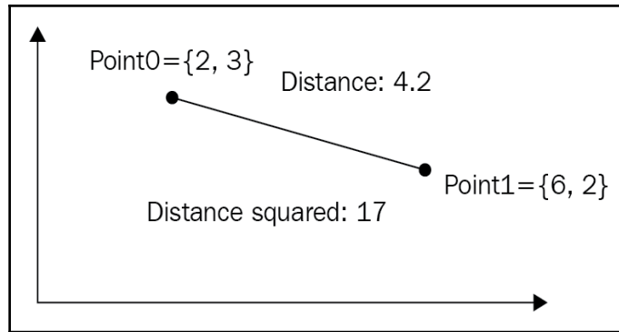
Distance, and squared distance between two points
