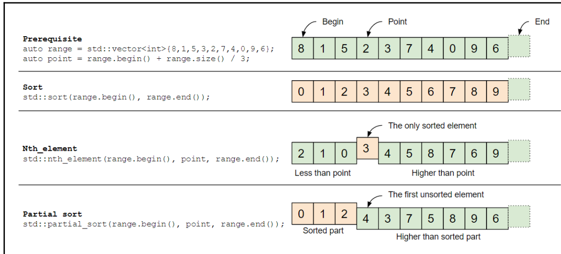
Sorted and non-sorted elements of a range using different algorithms
