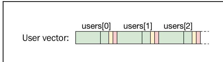
User objects stored contiguously in a vector
