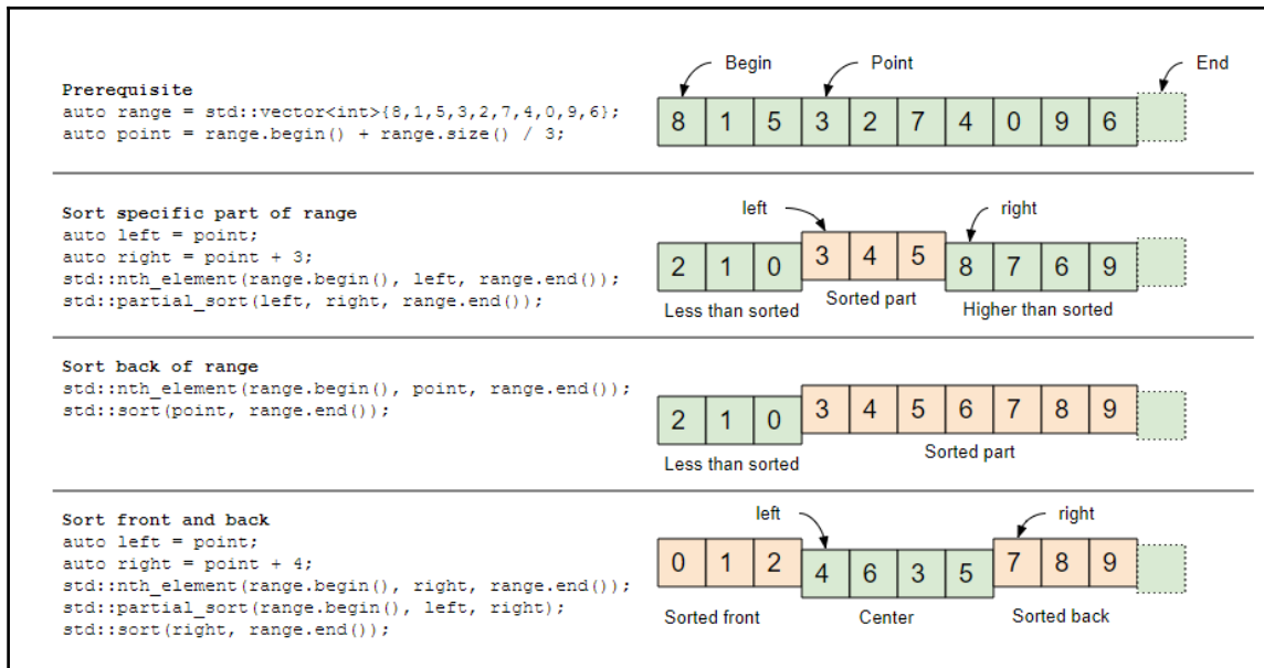
Combining algorithms and corresponding partially ordered result
