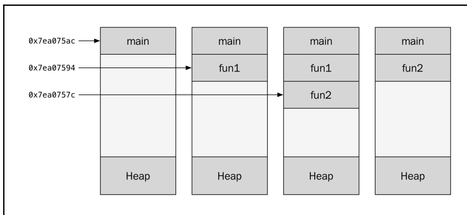
The stack grows and contracts when functions are entered and returns.
