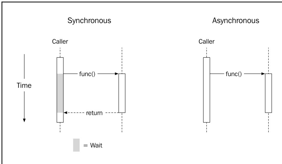
Synchronous versus asynchronous calls. The asynchronous task returns immediately but continue to work after the caller has regained control.
