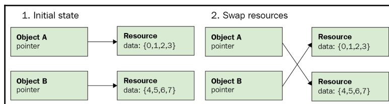
Swapping resources between two objects
