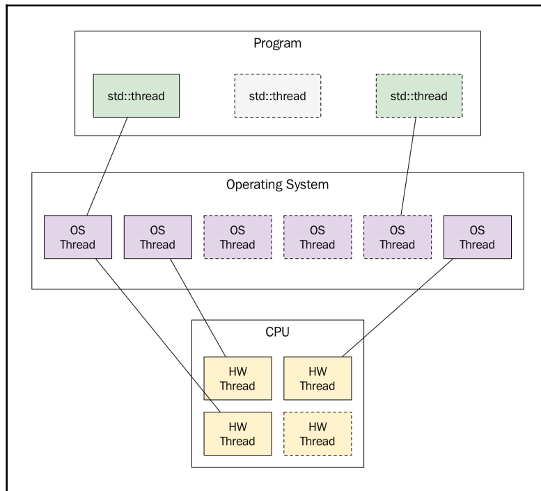
Snapshot of a hypothetical running system
