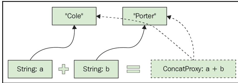
Proxy object representing an accumulation of two strings
