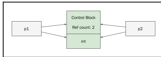
Two shared_ptr s accessing the same object
