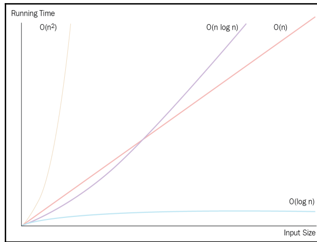
Comparison of growth rate functions
