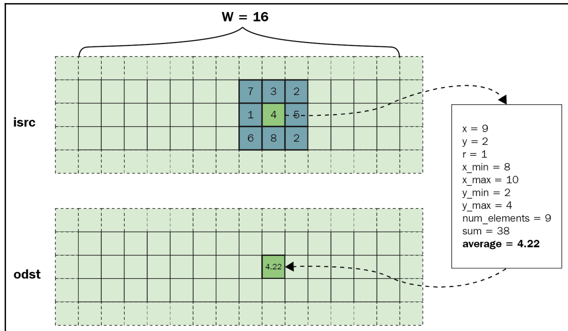
Box filter of an individual grid element
