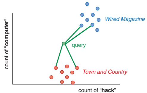
Figure C.1 Measuring Euclidean distance
