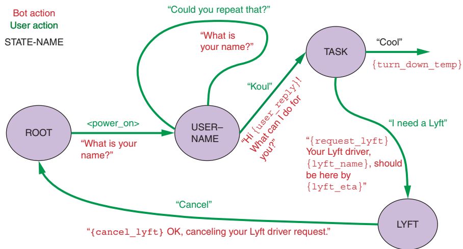
Figure 12.2 Managing state (context)
