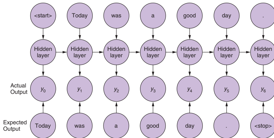
Figure 10.1 Limitations of language modeling
