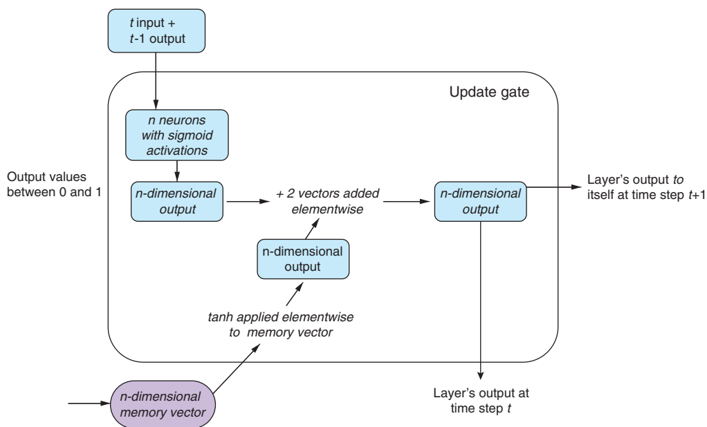
Figure 9.9 Update/output gate
