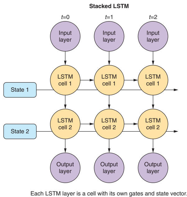
Figure 9.13 Stacked LSTM
