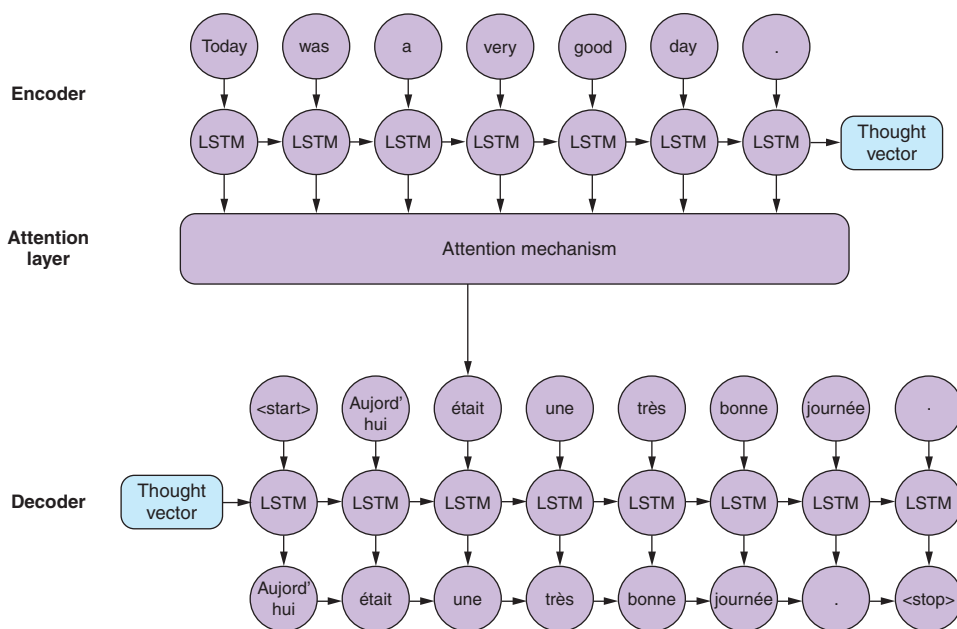
Figure 10.11 Overview of the attention mechanism
