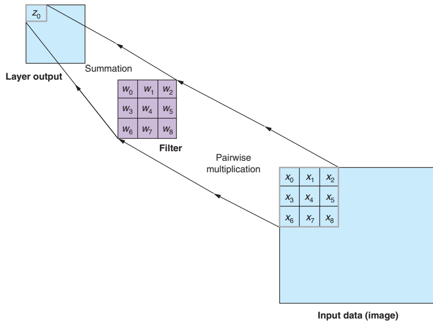
Figure 7.5 Convolutional neural net step
