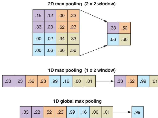
Figure 7.9 Pooling layers
