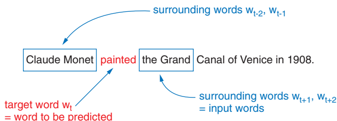
Figure 6.6 Training input and output example for the CBOW approach
