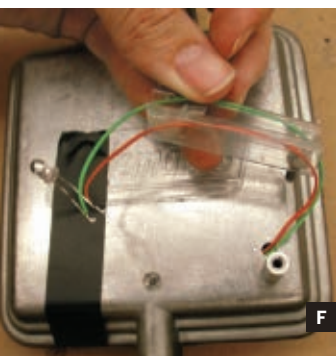
Fig. D: Test your optical pickup before installing. Fig. E: Drill holes in the case bottom for the power switch, indicator LED, output jack, and circuit board standoff. Fig. F: Drill the case top for the photo-
