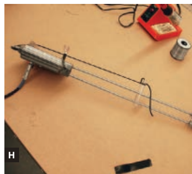
detector, then mount an arm to raise the emitter LED directly above it. Fig. G: The bridge is notched plastic tubing. Fig. H: The tuning head is more tubing that slides up or down the handles.
