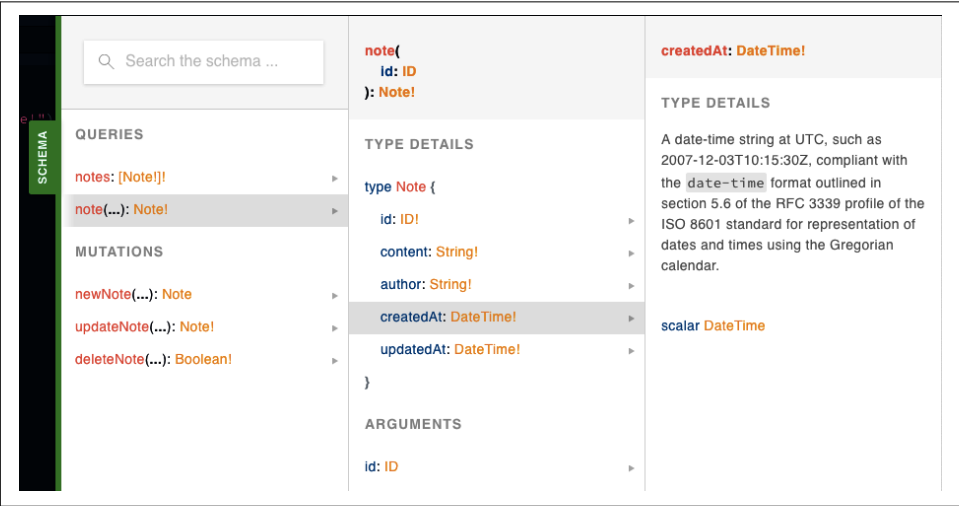
Figure 6-1. Our schema now features DateTime types
