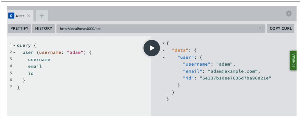
Figure 8-2. The user query in the GraphQL Playground
