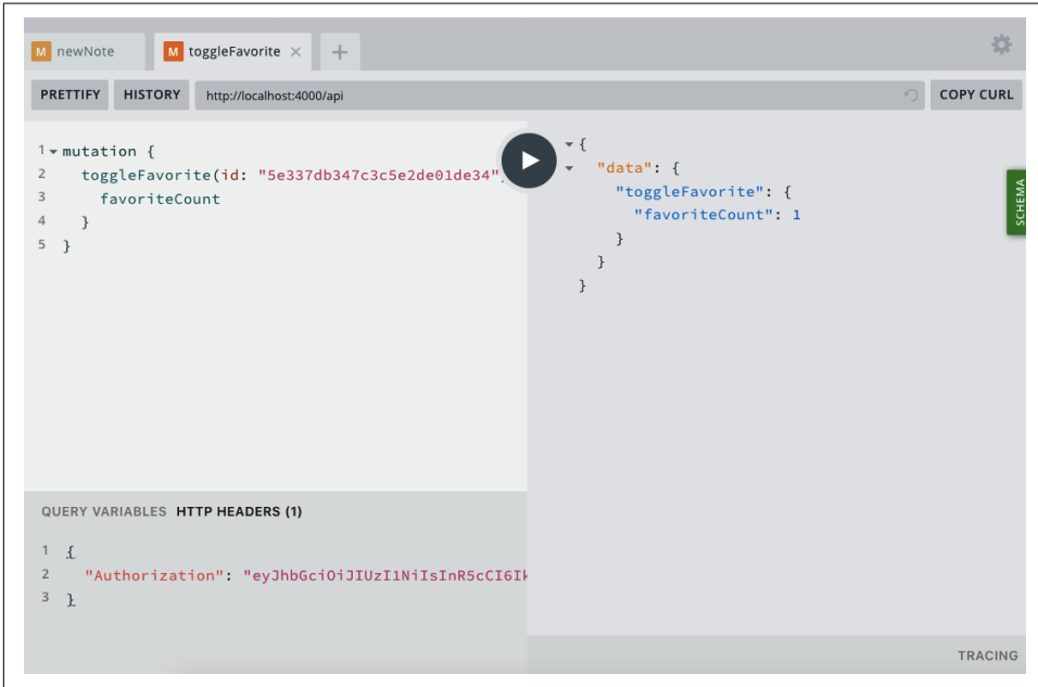
Figure 8-6. The toggleFavorite mutation
