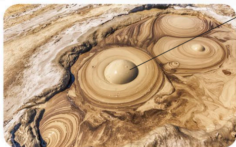
Mud volcano
