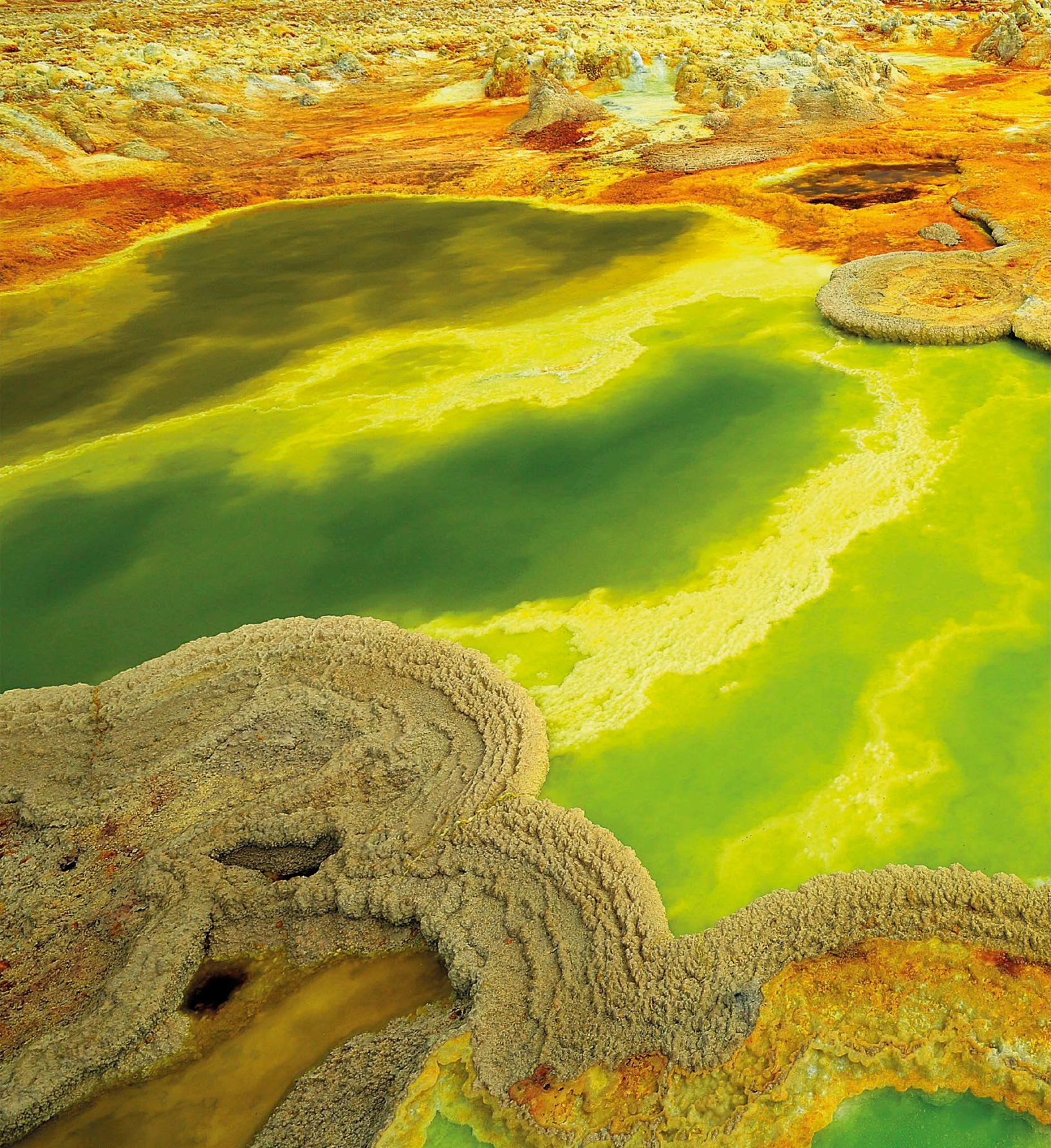
DANAKIL DEPRESSION This hot spring in Africa's Danakil Depression is surrounded by a yellow crust of pure sulfur. The sunken region between Ethiopia and Eritrea in East Africa is a wild volcanic area, packed with erupting craters, arid deserts, boiling mud, and pools with unusual colours caused by the presence of sulfur and many mineral salts.
