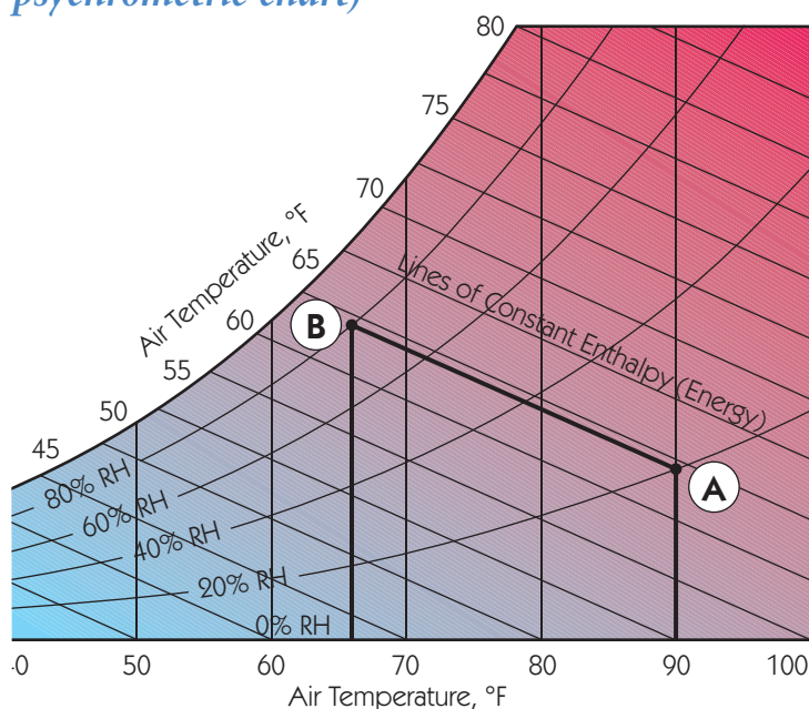
The Cooling Effect (as shown in a psychrometric chart)
