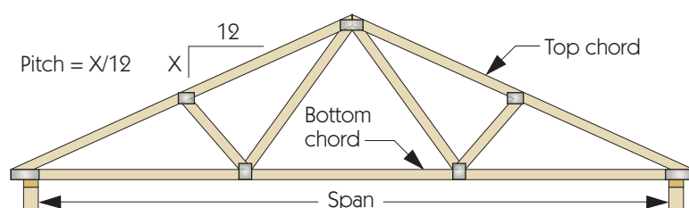
Fink Truss: 24" Spacing, 30 PSF Live, 7 PSF Dead
