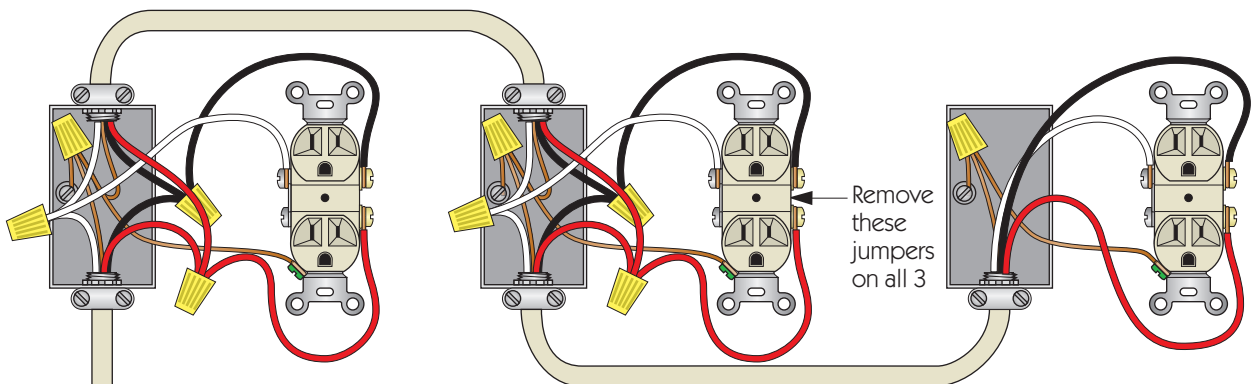
SPLIT-CIRCUIT RECEPTACLE (two separate circuits)
