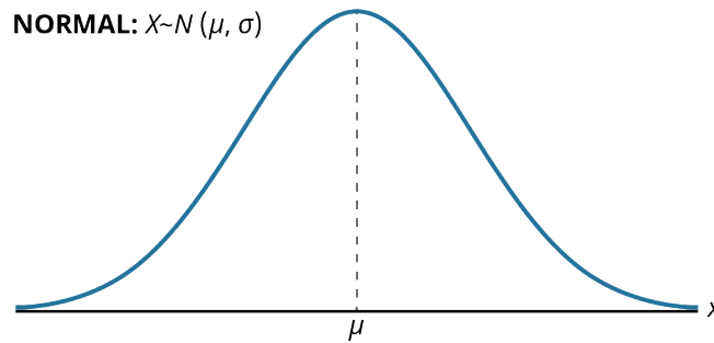
Figure 13.3 Graph of the Normal Distribution
