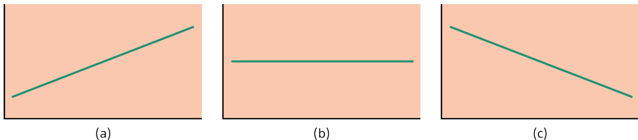
Figure 14.3 Three Possible Graphs of \hat{y} = a + bx (a) If b > 0 , the line slopes upward to the right. (b) If b = 0 , the line is horizontal. (c) If b < 0 , the line slopes downward to the right.
