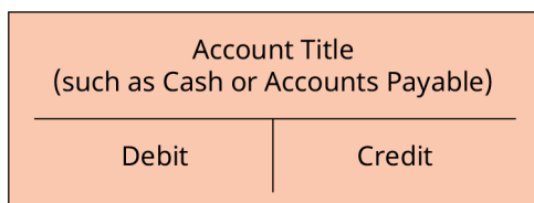
Figure 4.3 T-Account
