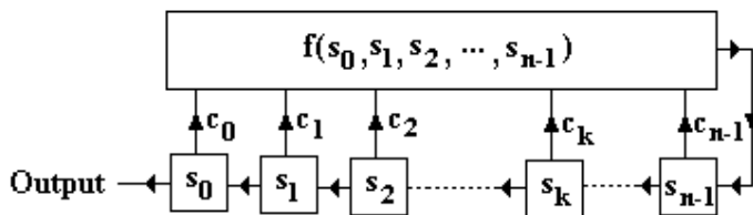
Gambar 20. Linear Feedback Shift Register (sumber: math.ucdenver.edu)
