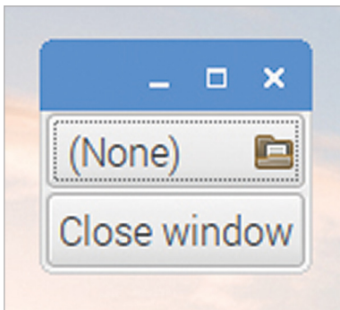
▲ A GtkFileChooserButton
