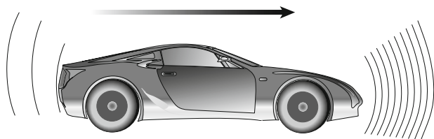
FIGURE 1.15 The sound waves emitted by a race car are affected by its speed, being crowded together in front of the car and spreading apart behind it, leading to the characteristic change in pitch as a moving object passes a listener.
