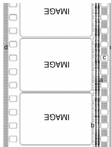
FIGURE 13.1 A representation of a release print showing the relative position for four types of soundtracks: (a) conventional stereo variable area in the standard analog soundtrack area next to the picture, (b) DTS time code located between the picture and the conventional soundtrack areas for synchronization of an external disc, (c) Dolby Digital between the perforations on the soundtrack side of the film, and (d) Sony Digital Dynamic Sound located outside the perforations on both sides of the film. Frame lines of a Cinemascope picture are shown for reference. A positive release print is the inverse of the negatives.
