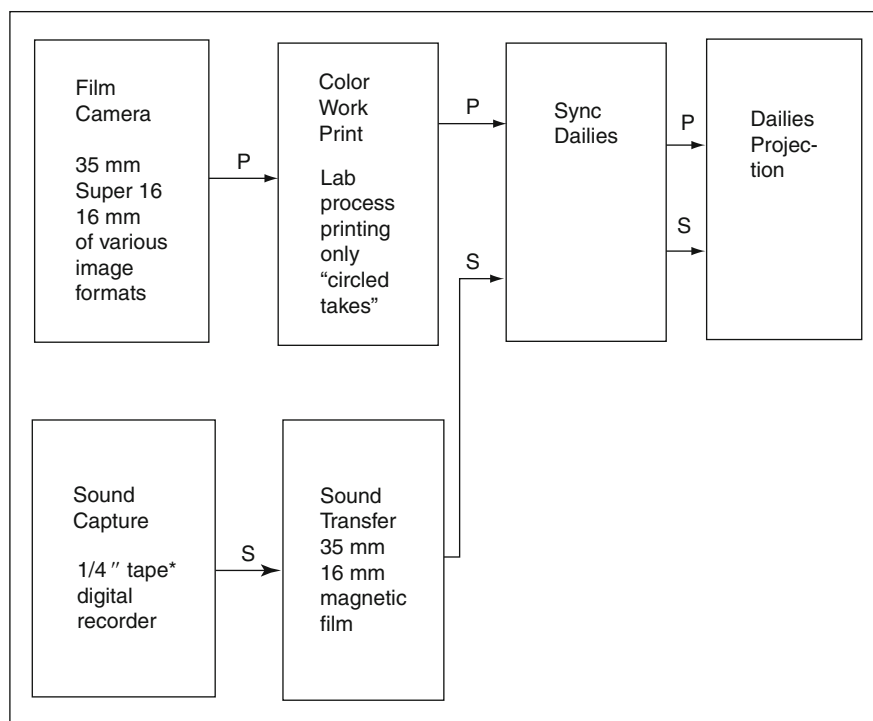
FIGURE 8.1 Conventional film capture, transfer, and dailies. Everything is at precisely 24 fps. The 1/4-inch tape has a time code or other reference that matches the camera frame rate.
