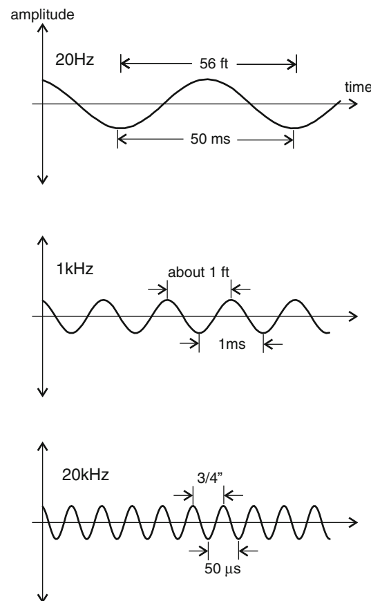
FIGURE 1.7 Wavelength and frequency of sound in air over the audible frequency range.
