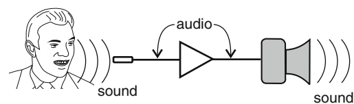
FIGURE 3.1 Audio is distinguished from sound by its being the electrical representation of sound, a physical phenomenon.
